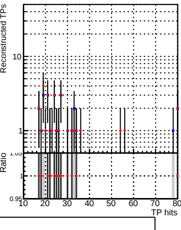
N of associated tracks (simToReco) vs hit
