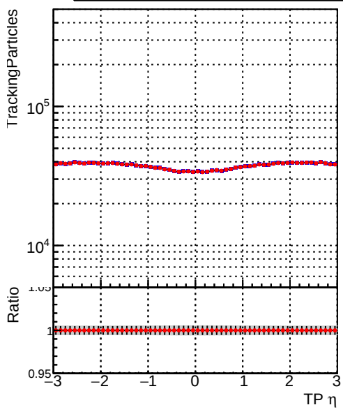
Legend: DQM_mkFit_TT_retrain-lowpt (blue circles), DQM_mkFit_TTold-lowpt (red circles)
