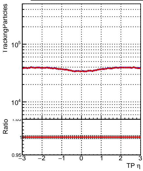
Legend: DQM_mkFit_TT_retrain-lowpt (blue squares), DQM_mkFit_TTold-lowpt (red circles)
