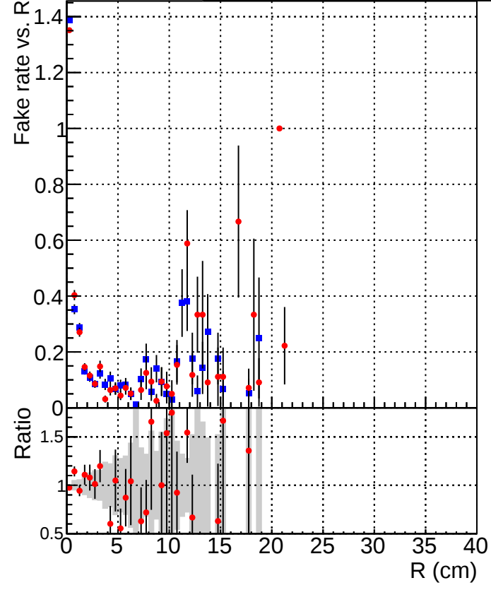
K_S^0 tracking fake rate vs R Legend: DQM_mkFit_TT_retrain-lowpt (blue squares) DQM_mkFit_TTold-lowpt (red circles)
