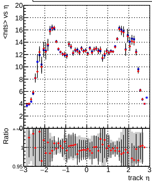
— DQM_mkFit_TT_retrain-lowpT — DQM_mkFit_TTold-lowpT mean hits > \eta
