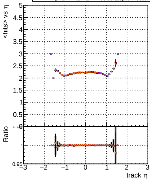
mean hit DQM_mkFit5_TTold-lowpt DQM_mkFit_TT_retrain-lowpt DQM_mkFit_TTold-lowpt DQM_mkFit_TT_NEWdefault_specPLess3-lowpt
