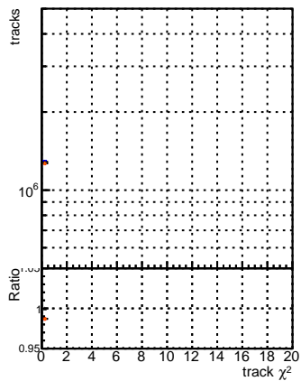
N of reco track vs. \chi^2 for different \chi^2 bins and \chi^2 sets
