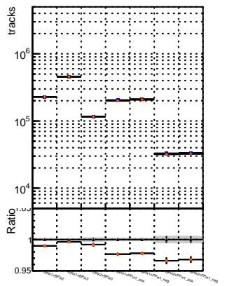
N of reco track vs. \chi^2 for different \chi^2 bins and \chi^2 sets
