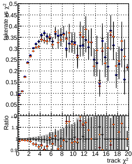
Fake rate vs. Legend: DQM mkFit5 Told lowpt Told lowpt NEW default specPLess3-lowpt
