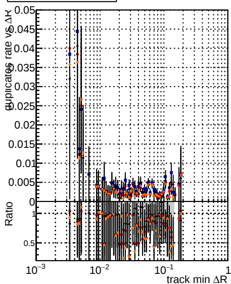
DOM mkeFit5 Told-lowpt DOM mkeFit5 Told-train-lowpt DOM mkeFit5 NEWdefault specPless3-lowpt
