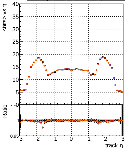
mean hit DQM_mkFit5_TTold-lowpt DQM_mkFit_TT_retrain-lowpt DQM_mkFit_TTold-lowpt DQM_mkFit_TT_NEWdefault_specPLess3-lowpt
