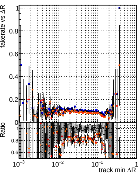
Fake rate vs \Delta R(\text{track, jet}) DQM mktFit5 Told-lowpt DQM mktFit5 Told-train-lowpt DQM mktFit5 Told-test-lowpt DQM mktFit5 Told-new-lowpt DQM mktFit5 Told-specPLEss3-lowpt
