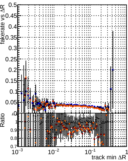
Fake rate vs \Delta R(\text{track, jet}) DQM mktFit5 Told-lowpt Told-train-lowpt DQM mktFit5 Told-train-lowpt DQM mktFit5 NEWdefault specPLe3-lowpt
