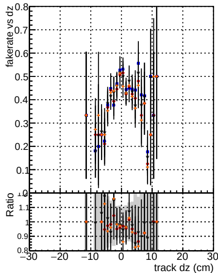
Fake rate vs d DQM mkt TT Told lowpt DQM mkt TT NEW default specPless3-lowpt
