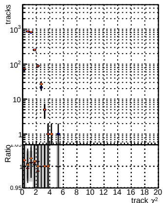
N of reco track vs. \chi^2 BSM mH E5 T Told-lowpt BSM mH E5 T Told-lowpt BSM mH E5 T Told-lowpt NEW default specPless3-lowpt
