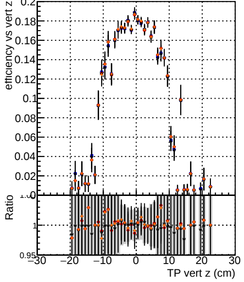
Efficiency vs. TP vert z — DQM_mkFit5_TTold-lowpt — DQM_mkFit_TT_retrain-lowpt — DQM_mkFit_TTold-lowpt — DQM_mkFit_TT_NEWdefault_specPLess3-lowpt
