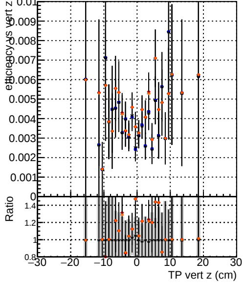
Efficiency vs. TP vert z (cm) DOM_mkFit5_TTold-lowpt DOM_mkFit_TT_retrain-lowpt DOM_mkFit_TTold-lowpt DOM_mkFit_TT_NEWdefault_specPLess3-lowpt
