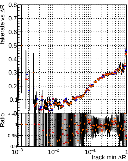
Fake rate vs \Delta R (track, jet) DOM mkeFit5 Told-lowpt Told-train-lowpt DOM mkeFit5 Told-lowpt specPLEss3-lowpt
