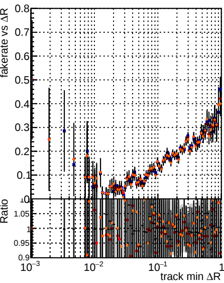
Fake rate vs \Delta R(\text{track, jet}) for various models and lowpt settings.
