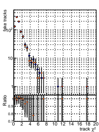
N of reco track vs. \chi^2 BDM mF5 Told lowpt BDM mF5 Told lowpt BDM mF5 Told lowpt NEWdefault specPless3-lowpt
