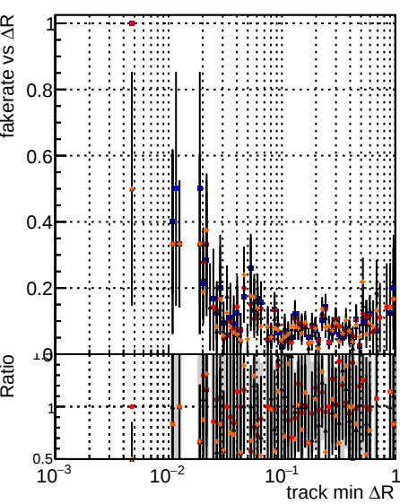
Fake rate vs \Delta R(\text{track, jet}) Legend: DOM (black) mkeFit5 (blue) Told-lowpt (red) Told-train-lowpt (orange) NEWdefault (grey) specPLe3-lowpt (black)
