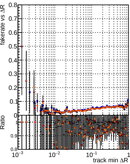
Fake rate vs \Delta R(\text{track, jet}) DQM mktFit5 Told-lowpt DQM mktFit5 Told-train-lowpt DQM mktFit5 Told-test-lowpt DQM mktFit5 Told-specPLEss3-lowpt
