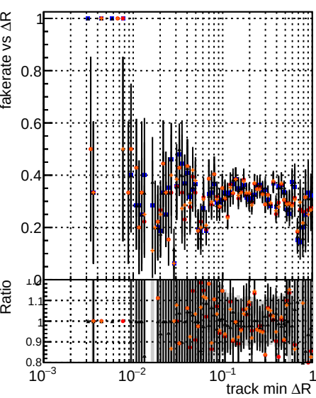
Fake rate vs \Delta R(\text{track, jet}) DOM mkeFit5 Told-lowpt DOM mkeFit5 Told-train-lowpt DOM mkeFit5 NEWdefault specPLeSS3-lowpt
