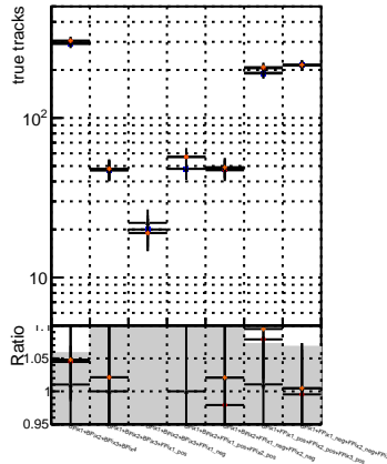
N of reco track vs. \chi^2 DOM E15 Told lowpt New default spec Pless3 lowpt
