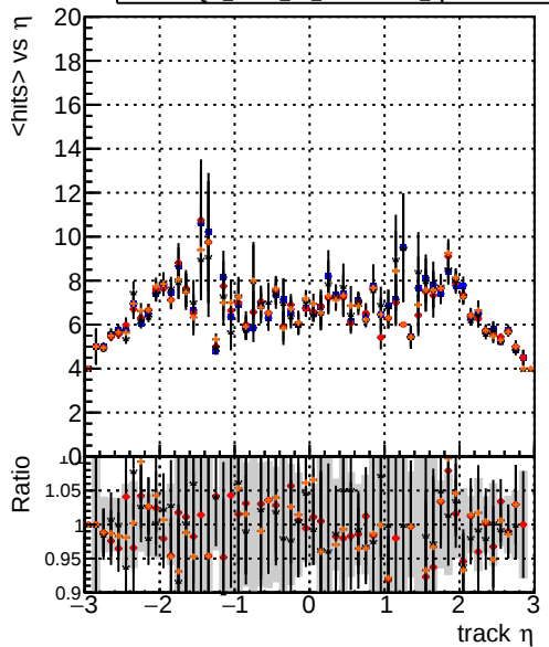
DQM_mkFit5_TTold-lowpt DQM_mkFit_TT_retrain-lowpt DQM_mkFit_TTold-lowpt DQM_mkFit_TT_NEWdefault_specPLess3-lowpt mean hit
