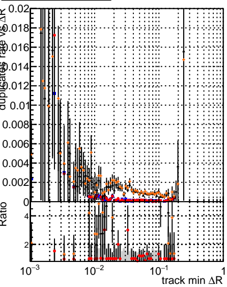
Legend for Fake rate vs \Delta R , Duplicates Rate vs \Delta R , and Pileup rate vs \Delta R : DQM mkFit5 Told-lowpt DQM mkFit5 Ttrain-lowpt DQM mkFit5 TOWS DQM mkFit5 NEWdefault specPLe3-lowpt
