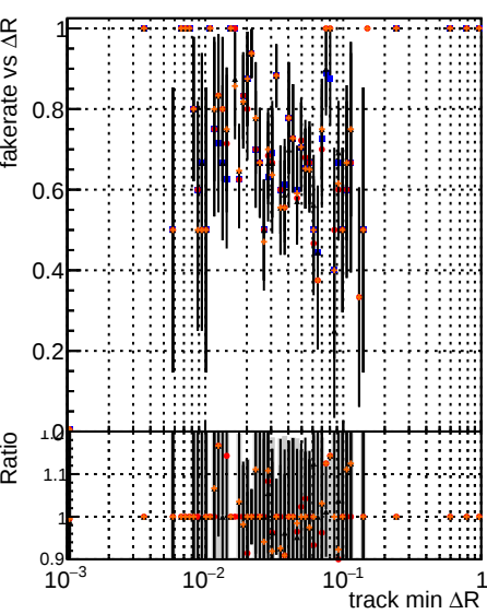
Fake rate vs \Delta R (track, jet) for various methods: DOM, mkeFit5, Told-lowpt, Told-train-lowpt, NEWdefault, specPLe3-lowpt
