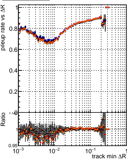
Legend for Fake rate vs \Delta R , Duplicates Rate vs \Delta R , and Pileup rate vs \Delta R : Blue line with dots: DQM mkFit5 TTold-lowpt Red line with dots: DQM mkFit5 Ttrain-lowpt Black line with dots: DQM mkFit5 TTold-lowpt Black line with dots: DQM mkFit5 Ttrain-lowpt Black line with dots: DQM mkFit5 NEWdefault specPLess3-lowpt
