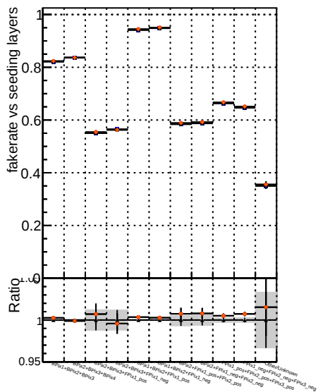
Fake rate vs. Legend: BQM mkl E5 TTold lowpt BQM mkl E5 TTol default spec Pless3 lowpt
