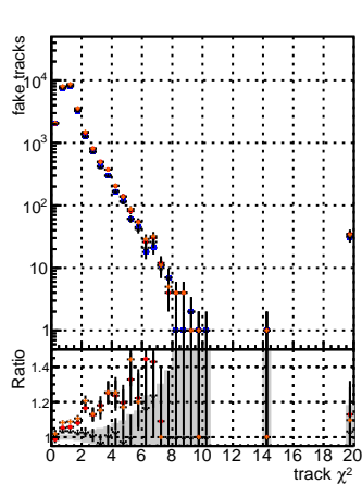
N of fake tracks vs. \chi^2 for different track sets
