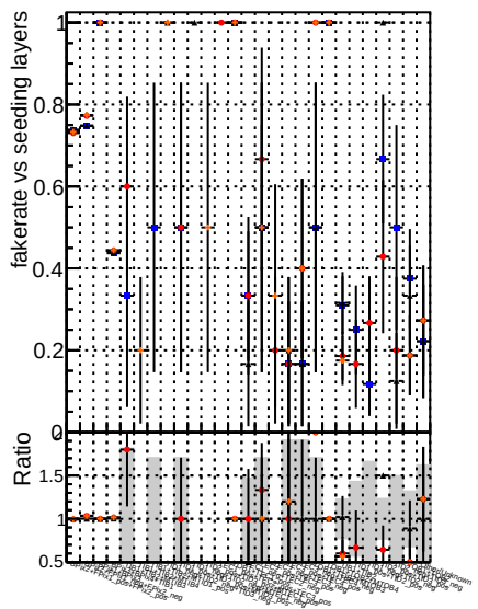
DOM mkFit5 Told lowpt DOM mkFit5 Told lowpt DOM mkFit5 Told lowpt NEW default specPLess3-lowpt Fake rate vs.
