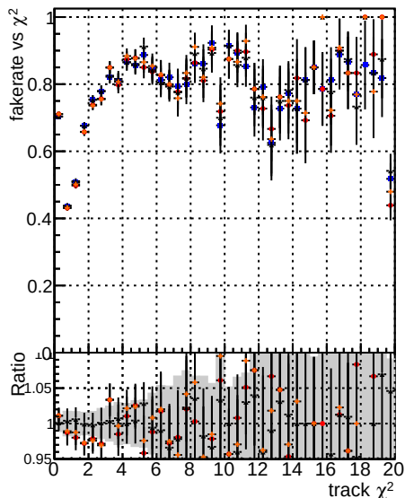
DOM mkFit5 Told lowpt DOM mkFit5 Told lowpt DOM mkFit5 Told lowpt NEW default specPLess3-lowpt Fake rate vs.
