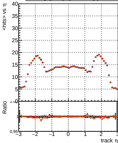
Legend: DQM_mkFit5_TTold-lowpt (blue line), DQM_mkFit_TT_retrain-lowpt (red line), DQM_mkFit_TTold-lowpt (black line), DQM_mkFit_TT_NEWdefault_specPLess3-lowpt (orange line) mean hits
