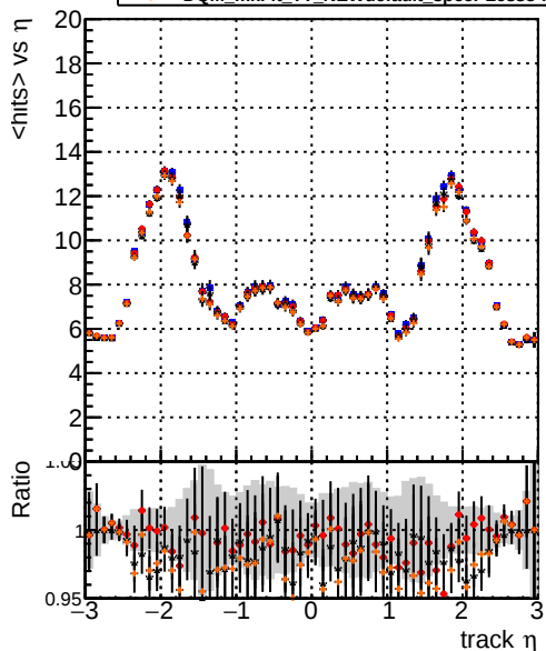
mean hits vs \eta DQM_mkFit5_TTold-lowpT DQM_mkFit_TT_retrain-lowpT DQM_mkFit_TTold-lowpT DQM_mkFit_TT_NEWdefault_specPLess3-lowpT
