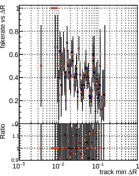
Fake rate vs \Delta R(\text{track, jet}) Legend: DOM (black) mkeFit5 (blue) Told-lowpt (red) Told-train-lowpt (orange) NEWdefault (grey) specPLeas3-lowpt (green)
