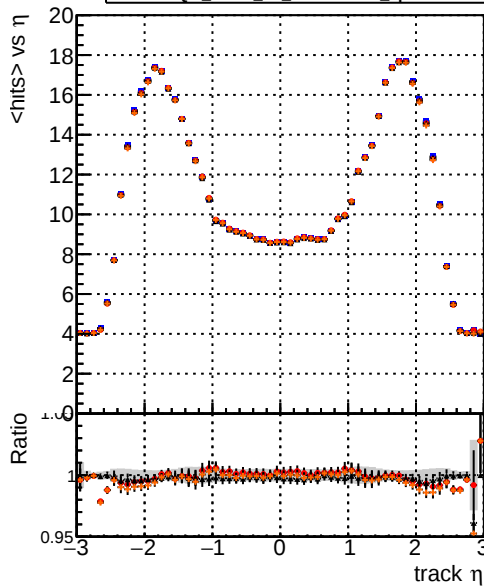
mean hit DOM_mkFit5 TTold-lowpt DOM_mkFit TT_retrain-lowpt DOM_mkFit TTold-lowpt DOM_mkFit TT_NEWdefault_specPLess3-lowpt
