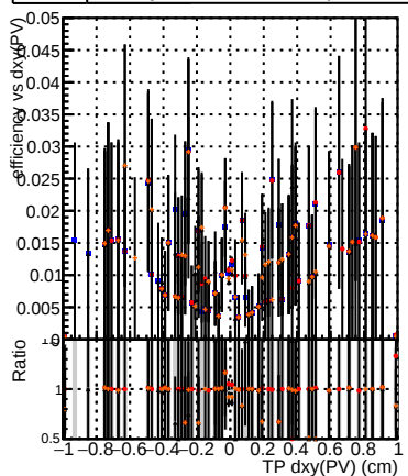
Efficiency —●— DQM_mkFit_TT_old-lowpT —●— DQM_mkFit_TT_NEWdefault_specPLess3-lowpT
