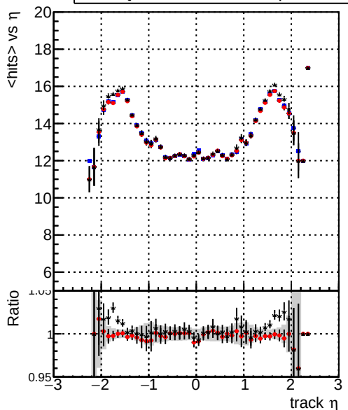
mean hits vs \eta — DQM_mkFit5_TTold-lowpt — DQM_mkFit_TT_retrain-lowpt — DQM_mkFit_TT_NEWdefault_specPless3-lowpt
