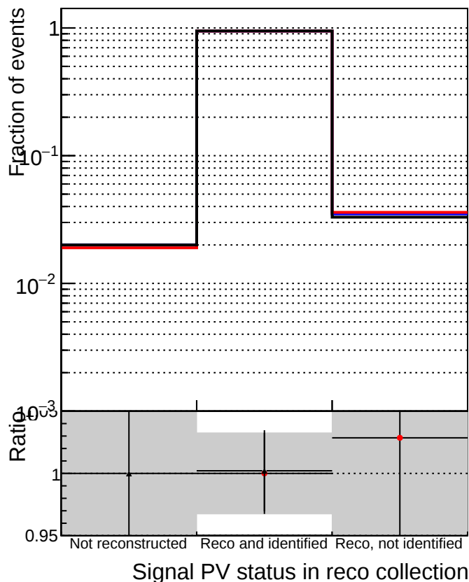
—■— DQM_mkFit5_TTold-lowpt —●— DQM_mkFit_TT_retrain-lowpt —*— DQM_mkFit_TT_NEWdefault_specPLess3-lowpt
