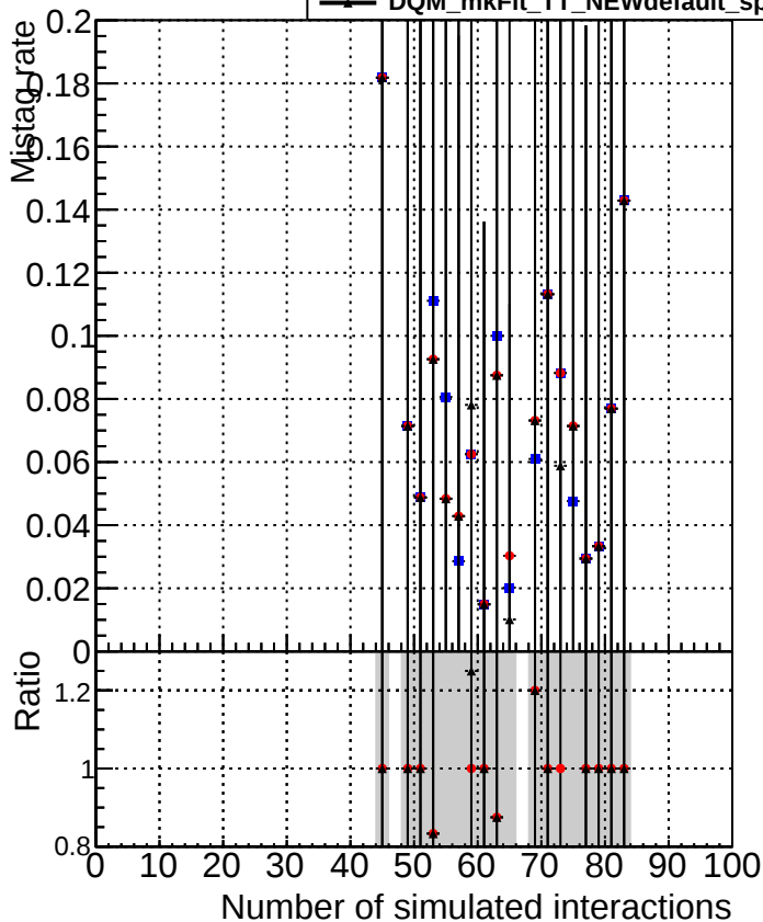
—■— DQM_mkFit5_TTold-lowpt —●— DQM_mkFit_TT_retrain-lowpt —*— DQM_mkFit_TT_NEWdefault_specPLess3-lowpt
