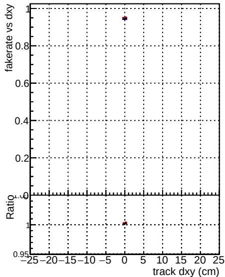
DOM mkFit5 TTold-lowpt DOM mkFit TT NEWdefault specPless3-lowpt
