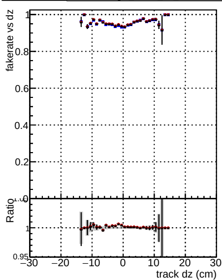
DOM mkFit5 TTold-lowpt DOM mkFit TT NEWdefault specPless3-lowpt
