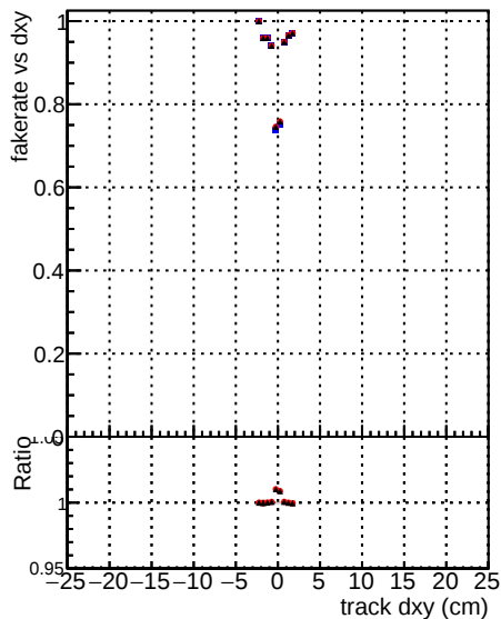
— DOM mkFit5 TTold-lowpt — DOM mkFit5 Tretain-lowpt — DOM mkFit5 TTNEWdefault specPless3-lowpt
