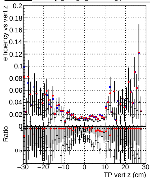
Efficiency vs. TP vert z (cm) — DQM_mkFit5_TTold-lowpt — DQM_mkFit_TT_retrain-lowpt — DQM_mkFit_TT_NEWdefault_specPless3-lowpt
