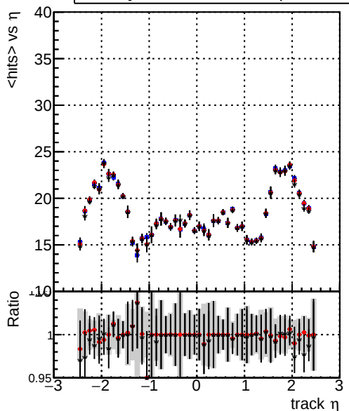
mean hit — DQM_mkFit5_TTold-lowpt — DQM_mkFit_TT_retrain-lowpt — DQM_mkFit_TT_NEWdefault_specPless3-lowpt
