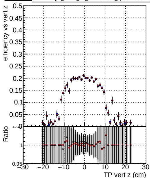
Efficiency vs. sim PV z — DQM_mkFit5_TTold-lowpt — DQM_mkFit_TT_retrain-lowpt — DQM_mkFit_TT_NEWdefault_specPLess3-lowpt
