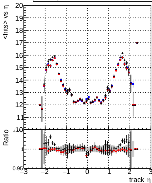
— DQM_mkFit5_TTold-lowpt — DQM_mkFit_TT_retrain-lowpt — DQM_mkFit_TT_NEWdefault_specPLess3-lowpt mean hits
