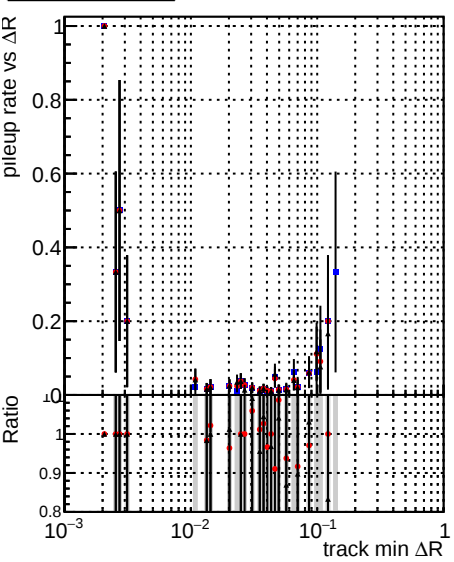
Legend: DQM_mkFit5_TTold-lowpt (blue), DQM_mkFit_TT_retrain-lowpt (red), DQM_mkFit_TT_NEWdefault_specPLeSS3-lowpt (black)
