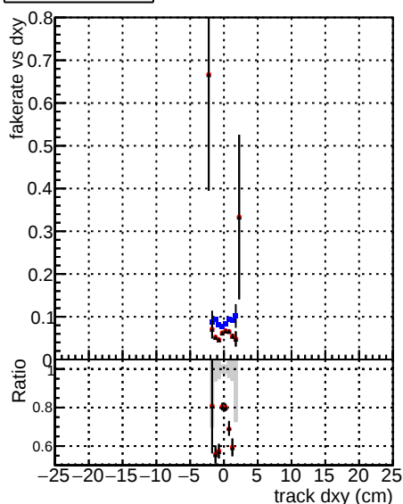
DOM mkFit5 TTold-lowpt DOM mkFit5 Tnew-lowpt DOM mkFit5 Tnew-lowpt specPless3-lowpt
