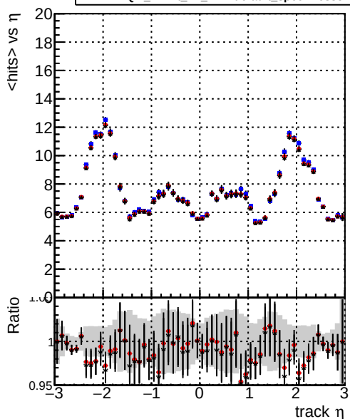
mean hit — DQM_mkFit5_TTold-lowpt — DQM_mkFit_TT_retrain-lowpt — DQM_mkFit_TT_NEWdefault_specPless3-lowpt
