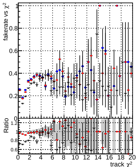
Fake rate vs. DOM mkFit5 Told-lowpt DOM mkFit NEWdefault specPless3-lowpt
