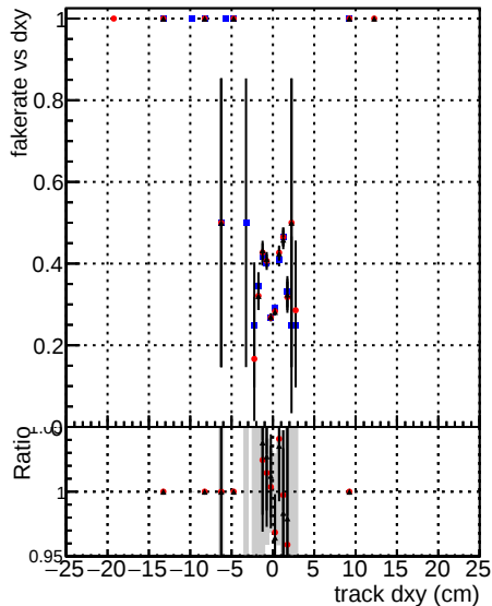
DOM mkFit5 TTold-lowp DOM mkFit5 Tretain-lowp DOM mkFit5 TNEWdefault specPless3-lowp
