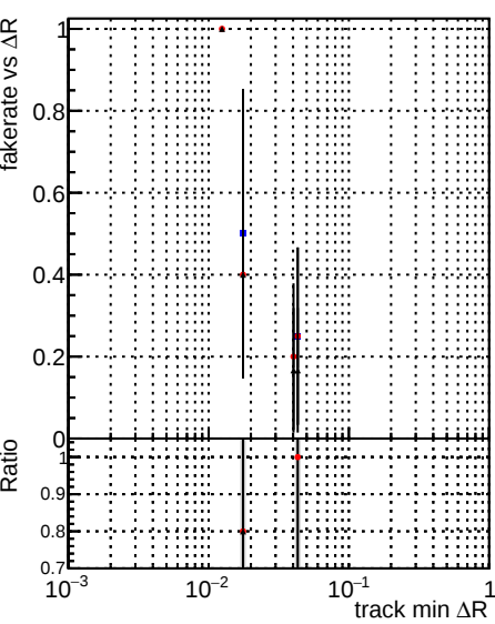
Fake rate vs \Delta R(\text{track, jet}) DQM_mkFit5_TTold-lowpt DQM_mkFit_TT_retrain-lowpt DQM_mkFit_TT_NEWdefault_specPLe3-lowpt
