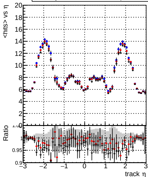
DQM_mkFit5_TTold-lowpt DQM_mkFit_TT_retrain-lowpt DQM_mkFit_TT_NEWdefault_specPLess3-lowpt mean hits
